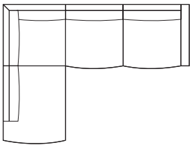
2,5- seater sofa with open-end LAMAR W 2570 x D 2230 x H 825 Loading ability- 32 pcs.
