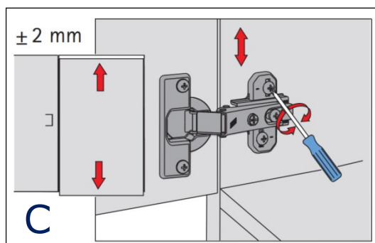
Height adjustment
