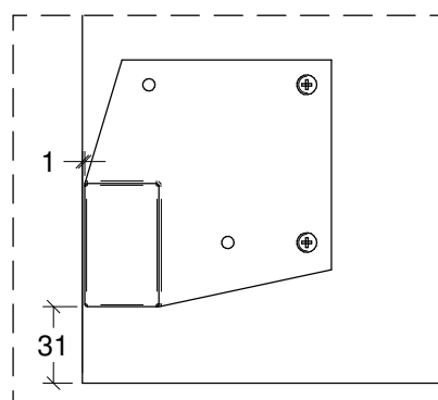
DETAIL 2
