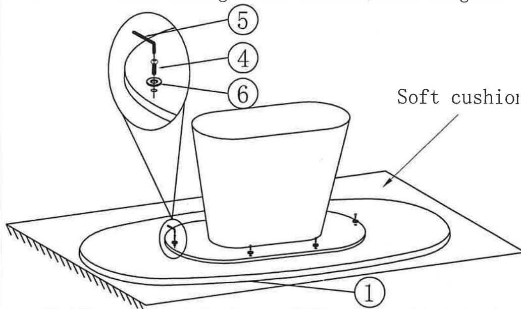
6527 Dining table installation diagram
