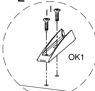
DETAIL 2
