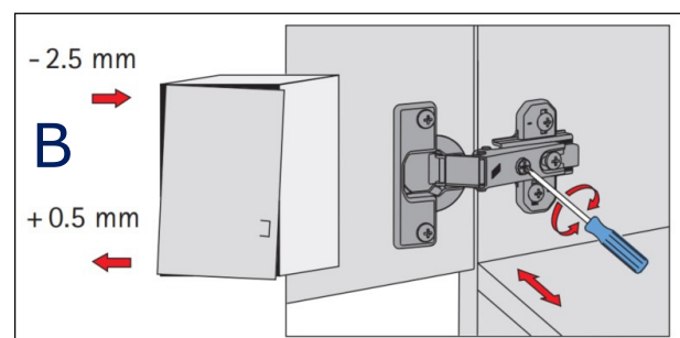
Overlay adjustment
