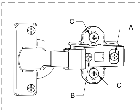
Depth adjustment
