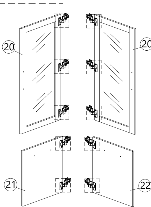
Inside View
