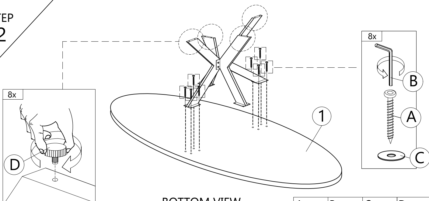
BOTTOM VIEW
