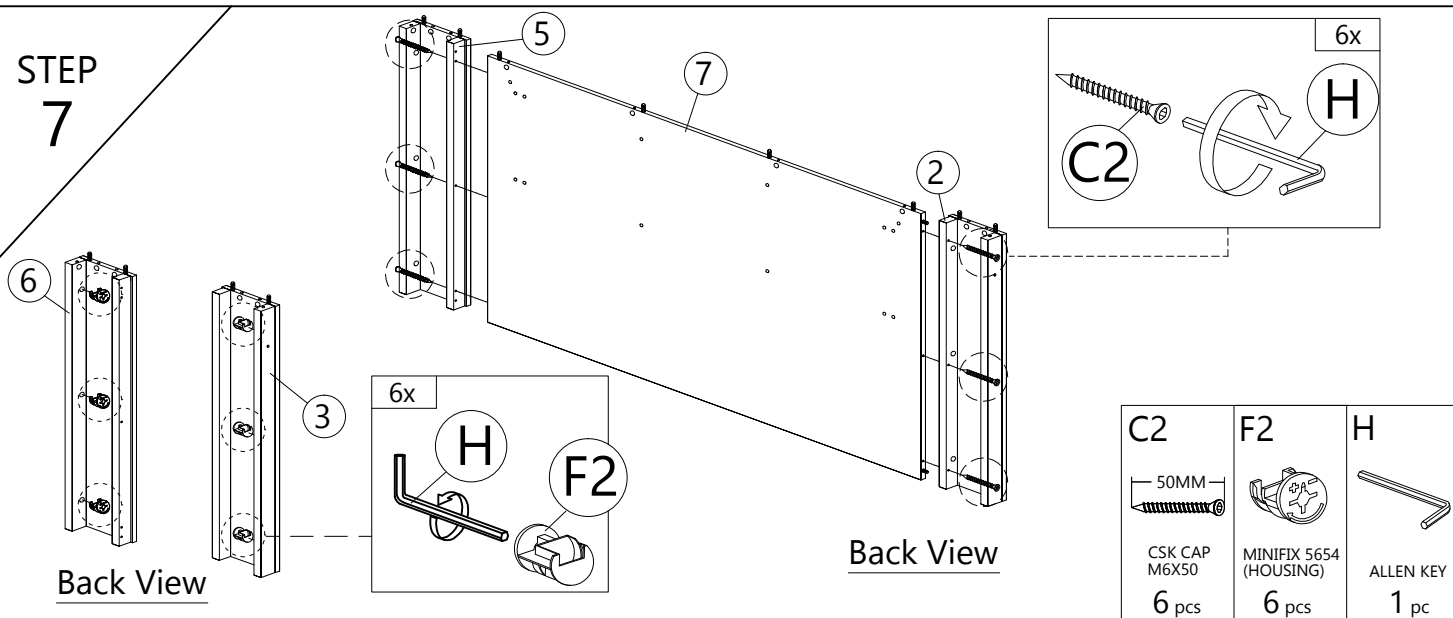
Back View
