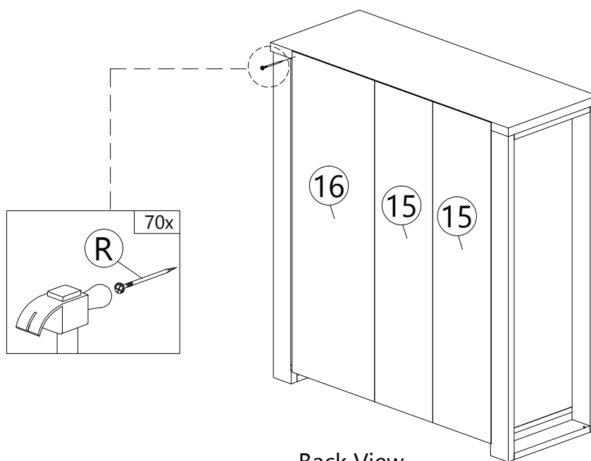
Back View
