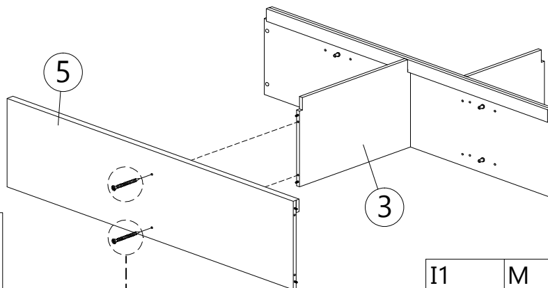
Left View
