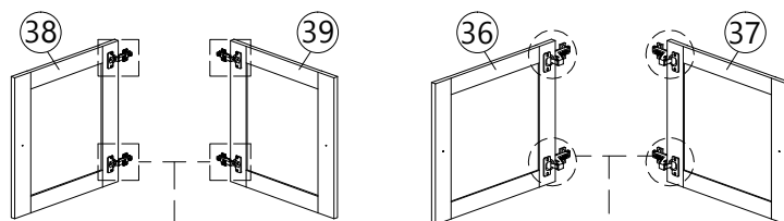
Outside View
