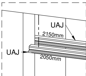
DETAIL 2
