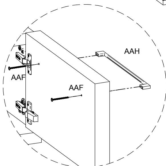
DETAIL 1
