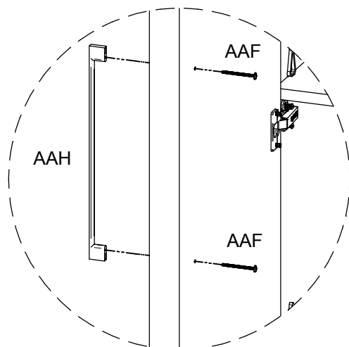
DETAIL 1
