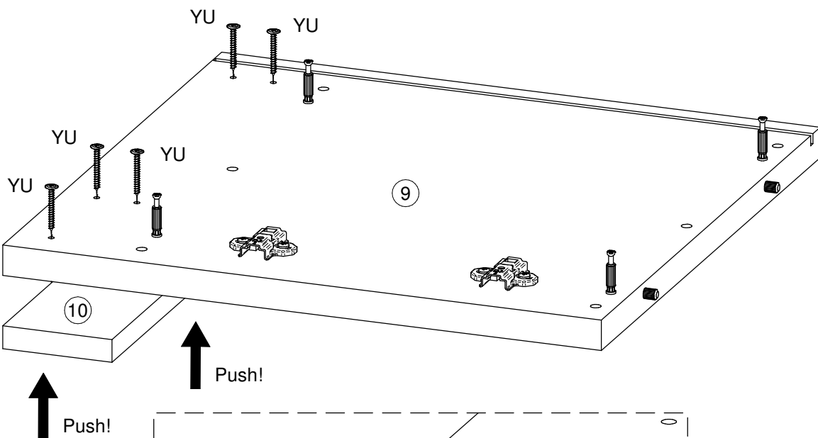
DETAIL 1
