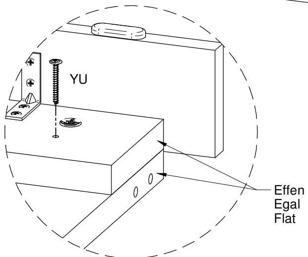
DETAIL A
